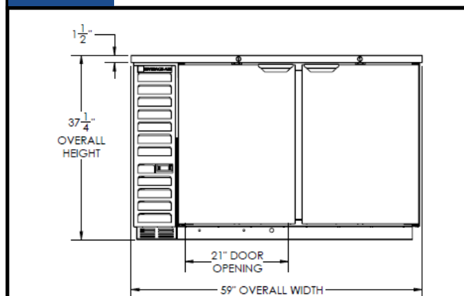
Elevation View
